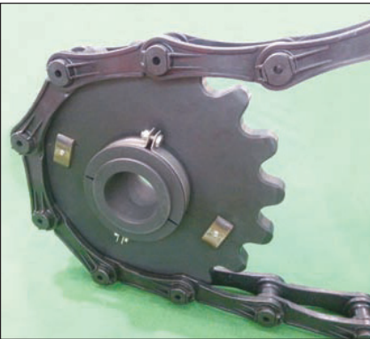
NM720S 带 F-228 / F-226 附件传动链 NM720S DRIVE CHAIN WITH F-228 / F-226
