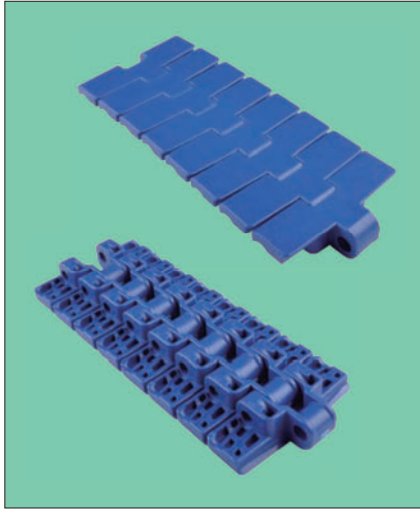
783M 平板型磁性转弯链 783M FLAT TOP MAGNET SIDEFLEXING CHAIN
